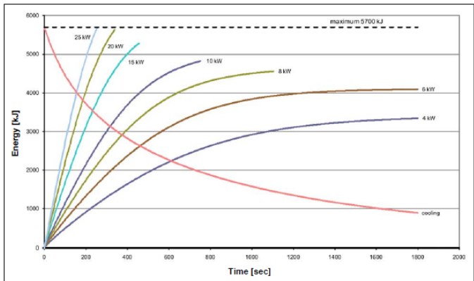
Fig. 7: The anode heating and cooling curves show the maximum heat content/capacity of the X-ray tube.
