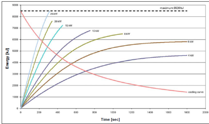
Fig. 8: The heating and cooling curves include the heat capacity of the cooling unit.
